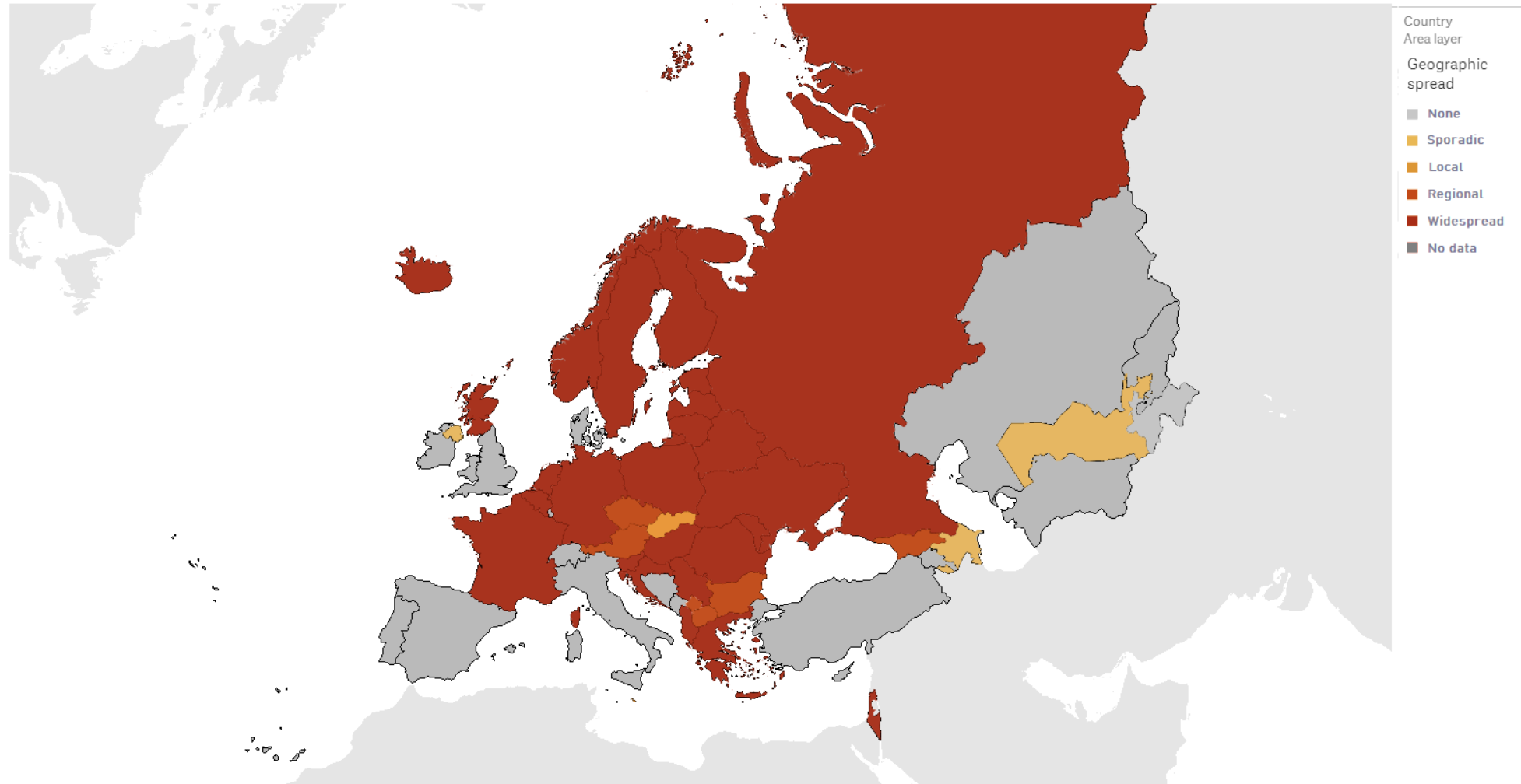
Geographic spread of influenza activity (EU layout map), 2023-W06
